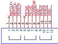
J3 12P_Cable
