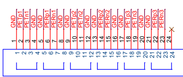
J4 24P_Cable
